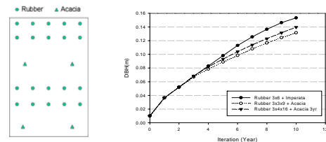
Figure 11. Double row rubber planting patterns 3x3x9 and 3x4x16 with Acacia between double rows of rubber (left) and its simulation output (right).
