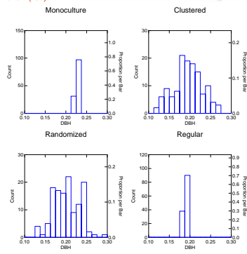
Figure 7. Size distribution of Rubber trees after 15 years of simulation.
