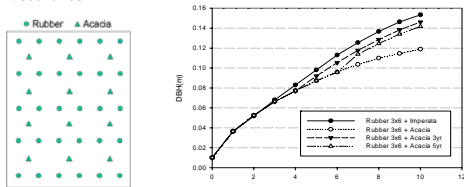
Figure 10. Rubber plantation 3x6m with alternating Acacia rows (left) and the simulation output (right).
