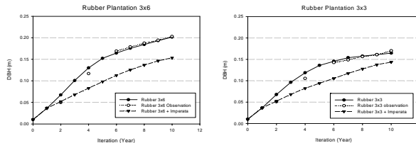
Figure 9 (left graph) shows the effect of Imperata on Rubber growth, the harvest size (15cm DBH) is delayed by about five years, and this is close to the observations at ICRAF experiments in West Kalimantan. Increasing the plot density to 3x3 spacing does not reduce Imperata effect (right graph).
