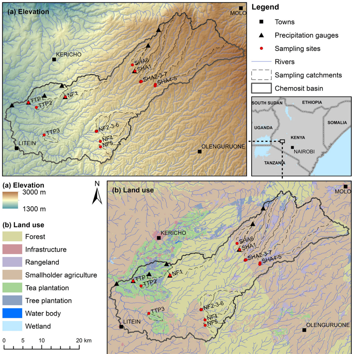
Fig. 1. Maps of the study area in the South-West Mau, Kenya, showing (a) elevation (SRTM digital elevation model 30 m resolution; USGS, 2000), and (b) land use classification based on Landsat imagery from 2013 (Swart, 2016). Precipitation gauges, sampling sites and catchments within the Chemosit basin are indicated on both maps. Labels refer to the sampling site and corresponding land use: NF = natural forest, SHA = smallholder agriculture and TTP = tea and tree plantations.
