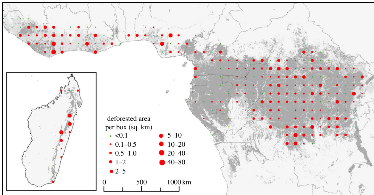
Figure 3. Net deforestation between 1990 and 2000. The circle size is proportional to the surface affected by deforestation in each sample of 100 km 2 .
