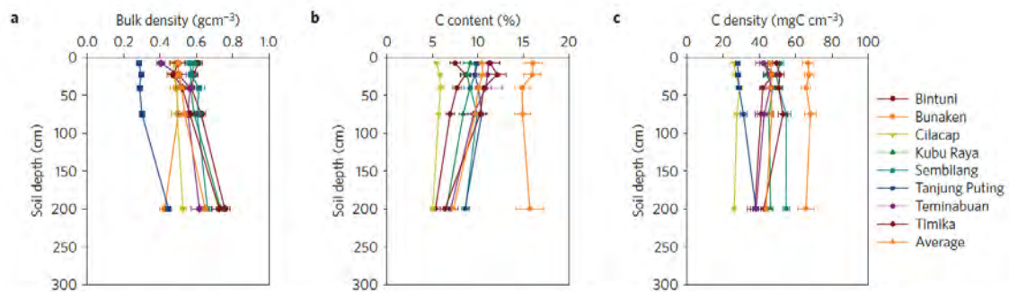
Figure 1 | Averaged values of soil properties. Soil bulk density (a), soil carbon content (b) and soil carbon density (c) of mangroves by depth from eight regions of Indonesia. Horizontal bars signify the standard error.
